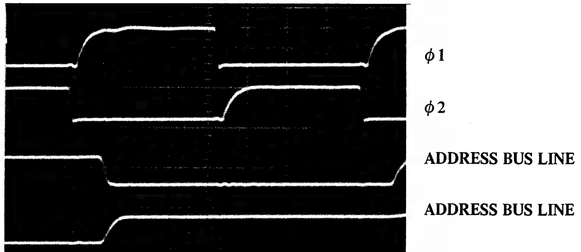
FIGURE 3.7a – Proper Address Lines
